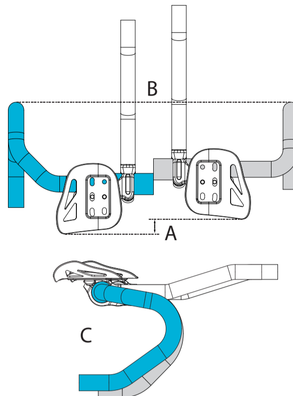
Largo drop bar compared to conventional drop bar
